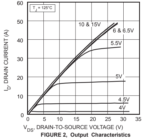
FIGURE 2, Output Characteristics
