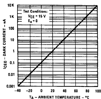
Dark Current vs Free Air Temperature
